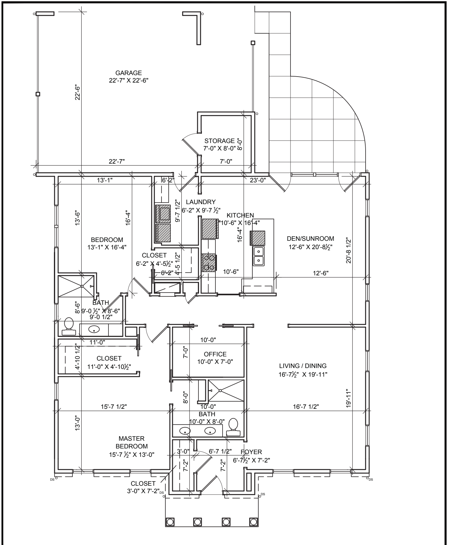
Asbury Floor Plan 1,880 Square Feet
